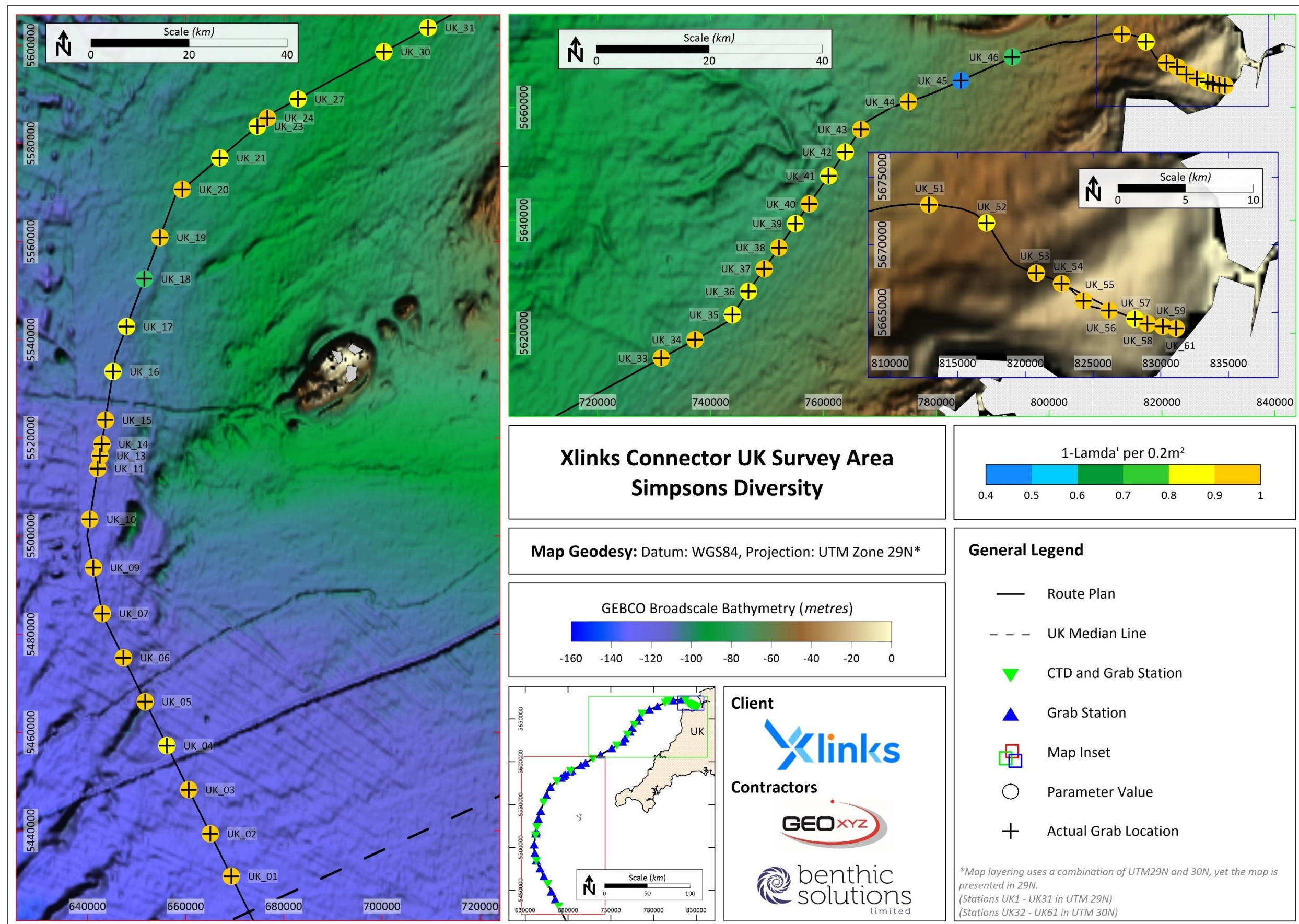
Figure 39: Macrofauna Simpson's diversity (1-lambda') per 0.2 m 2
