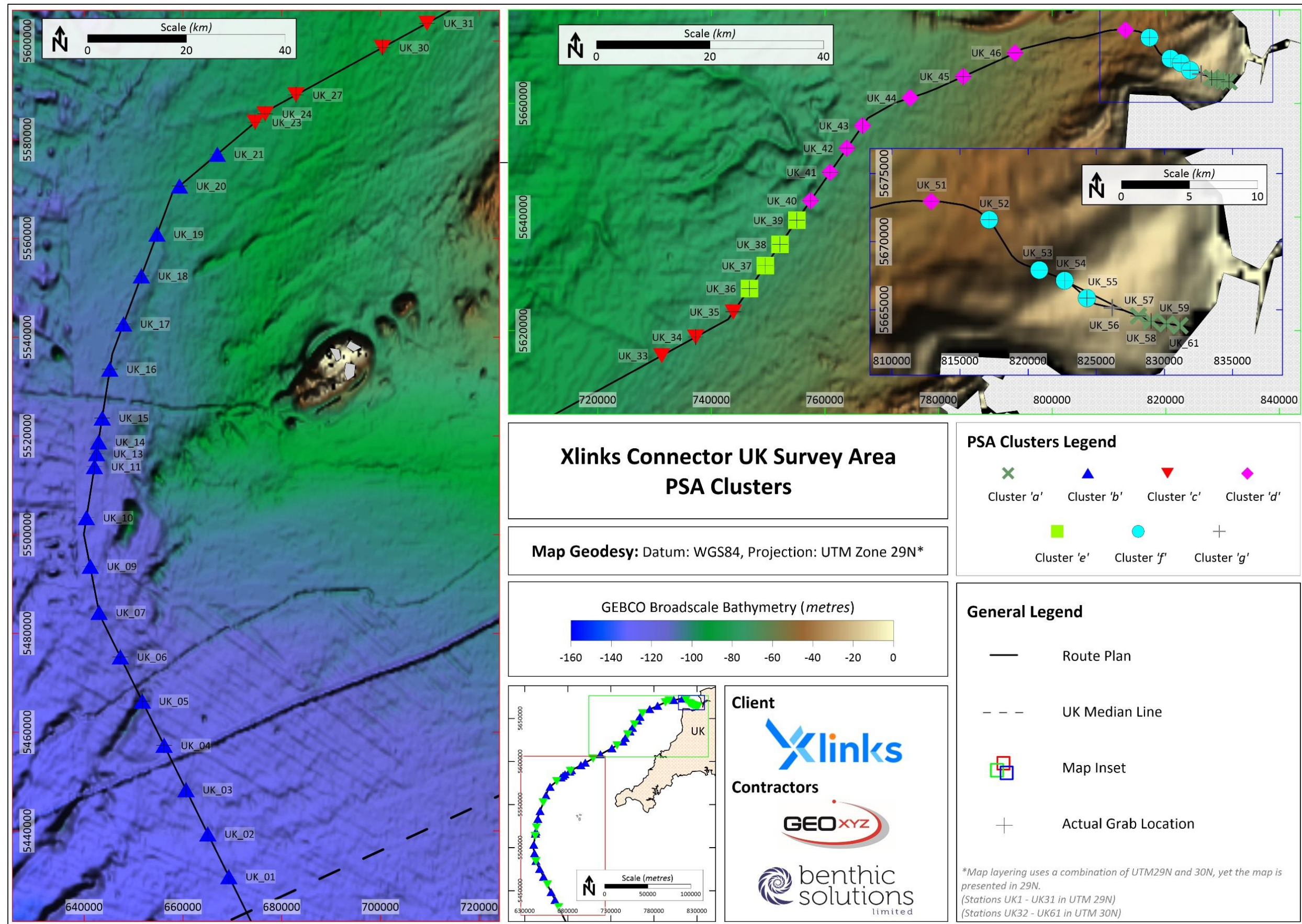
Figure 18: Multivariate PSD cluster distribution over MBES
