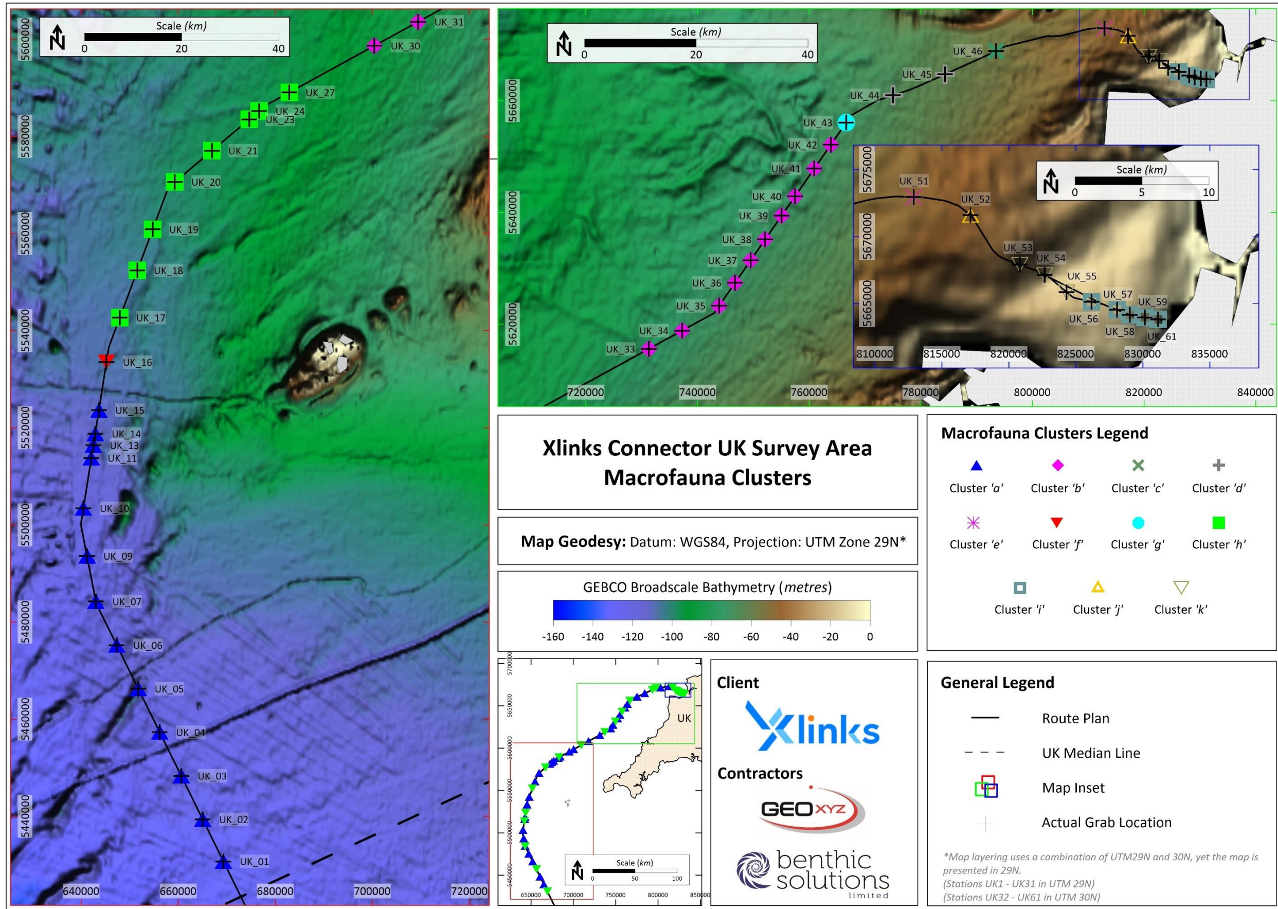
Figure 44: Macrofauna SIMPROF groups
